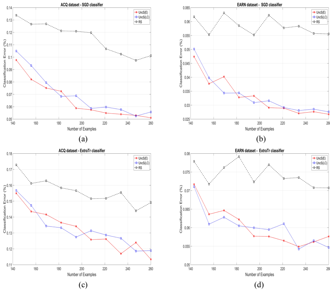
Fig. 1. Learning curves of SGD classifier (plots a and b) and ExtraTr classifier (plots c and d) for ACQ and EARN datasets for both Uncertainty methods along with Random sampling.
